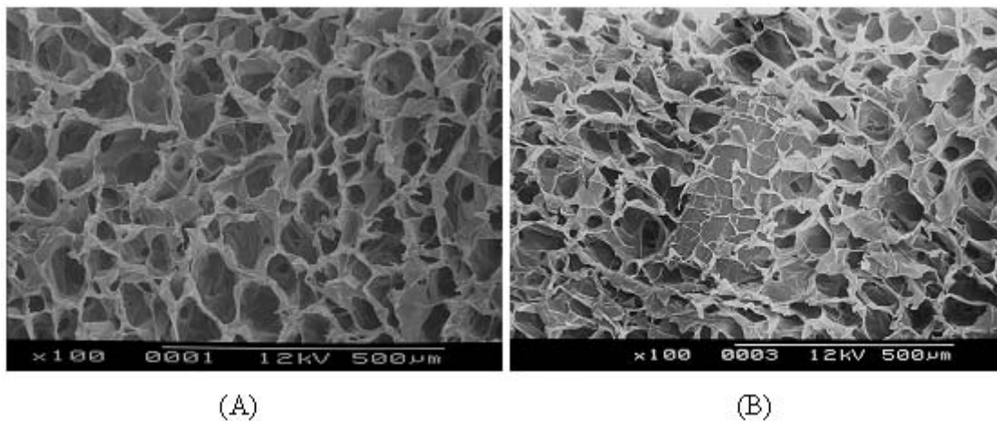
Figure 3. SEM photographs of cross-sectioned scaffolds: (A) chitosan and (B) demineralized bone matrix/chitosan.
