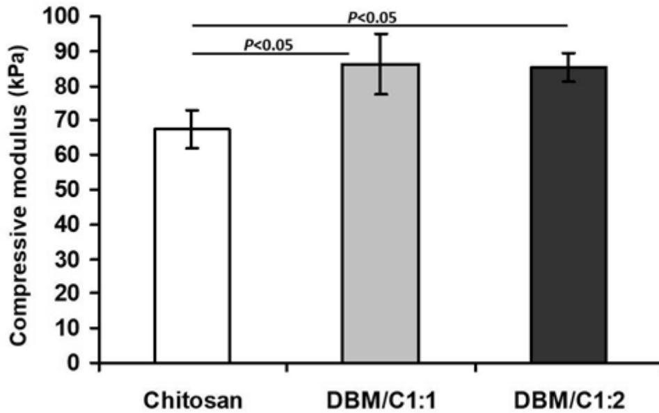
Figure 1. Compressive modulus of chitosan and demineralized bone matrix/chitosan (DBM/C) scaffolds.
